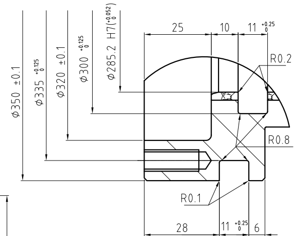
DETAIL B
